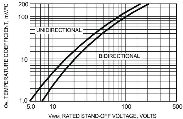
FIG. 11 - BREAKDOWN VOLTAGE TEMPERATURE COEFFICIENT CURVE
