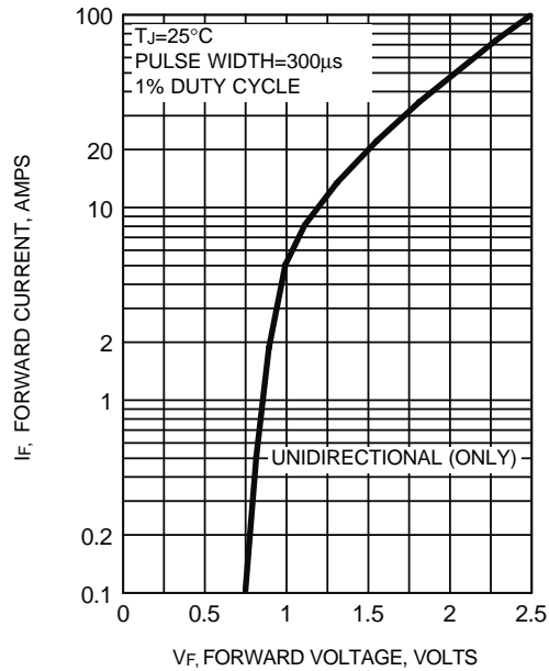
FIG. 10 - TYPICAL INSTANTANEOUS FORWARD VOLTAGE CHARACTERISTICS CURVE
