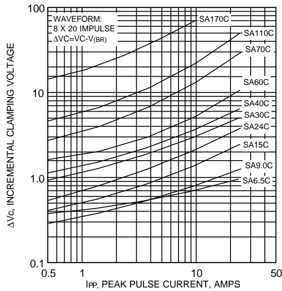
FIG. 8 - INCREMENTAL CLAMPING VOLTAGE CURVE BIDIRECTIONAL
