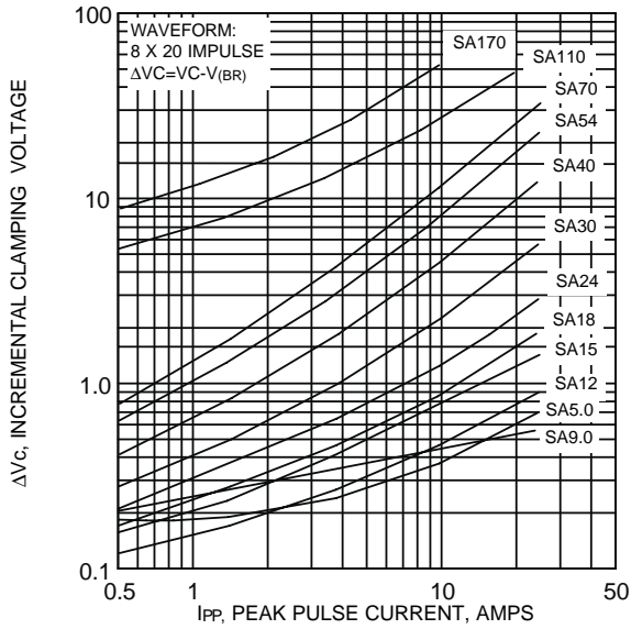
FIG. 6 - INCREMENTAL CLAMPING VOLTAGE CURVE UNIDIRECTIONAL
