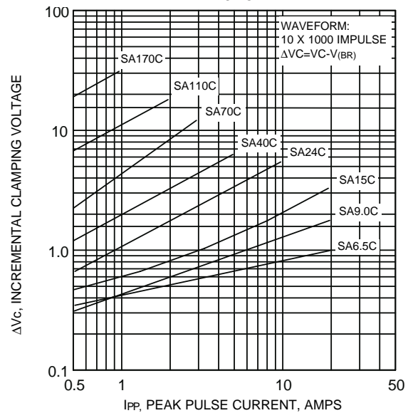
FIG. 9 - INCREMENTAL CLAMPING VOLTAGE CURVE BIDIRECTIONAL
